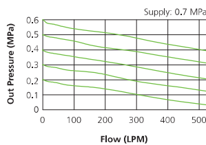
YT-200 / YT-205 Flow (LPM)
